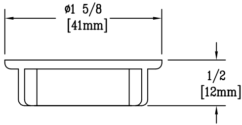
LOCKNUT
