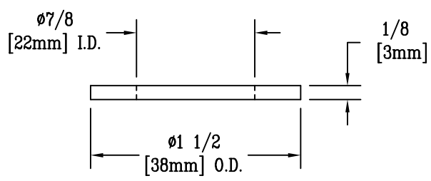
LOCK WASHER
